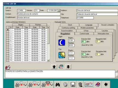
Programming the LRF-04
